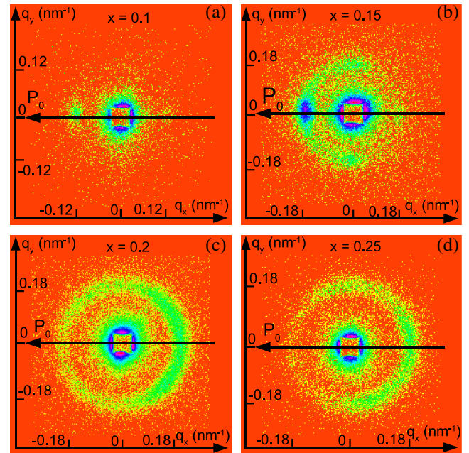
FIG. 2 (color online). Maps of the polarized SANS intensities for \mathbf{P}_0 along the guide field of \text{Fe}_{1-x}\text{Co}_x\text{Si} with x = 0.10 (a), x = 0.15 (b), x = 0.20 (c), x = 0.25 (d). The maps (a) and (b) show the left chirality, but samples at (c) and (d) are right handed.
