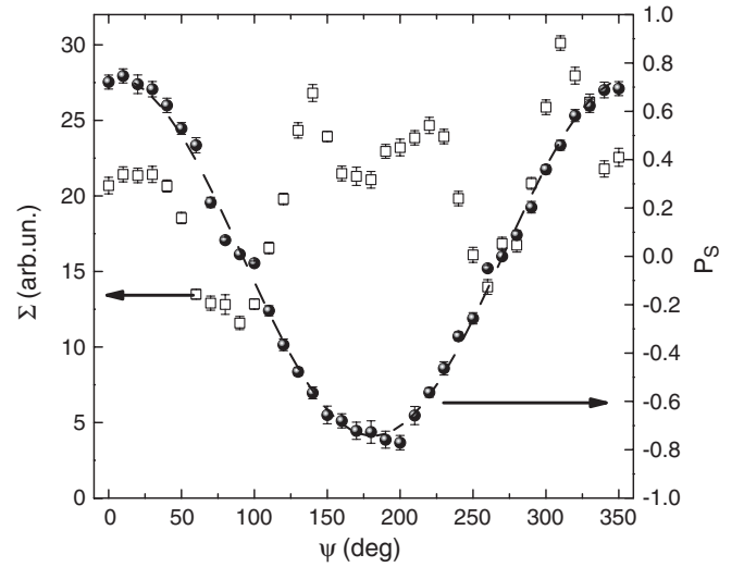
FIG. 4. Dependence of the scattering intensity \Sigma and the value P_s on the azimuth angle \psi seen anticlockwise from the horizontal axis for the compound with x = 0.2 .
