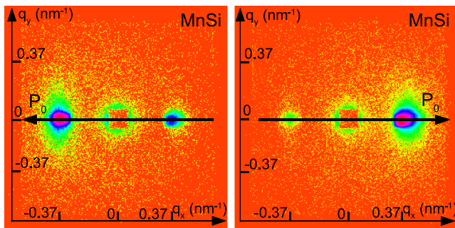
FIG. 1 (color online). Maps of the polarized SANS intensities of MnSi for the polarization \mathbf{P}_0 along the guide field (left) and opposite to it (right) at T = 25 K.
