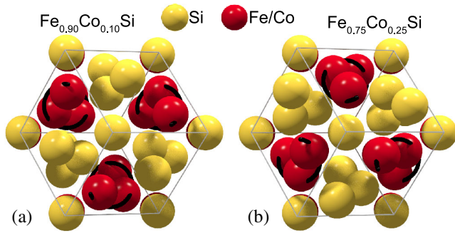
FIG. 5 (color online). The view of the B20 structure along the (111) axis for the sample with x = 0.10 (a) and x = 0.25 (b). The chirality of the metal sublattice is left handed for x = 0.10 and right handed for x = 0.25 . The black spirals help to identify the sense of the skewing.
