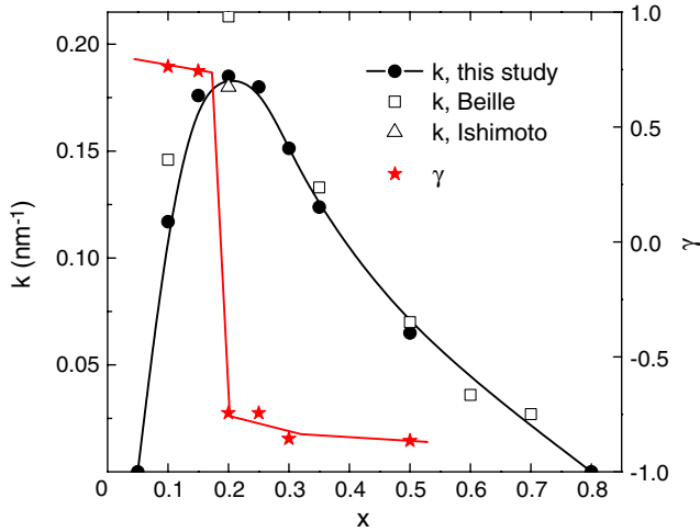
FIG. 3 (color online). Dependence of the helix wave vector k and the chirality \gamma on the Co concentration x for \text{Fe}_{1-x}\text{Co}_x\text{Si} ( \square [5], \triangle [6], \bullet this study).
