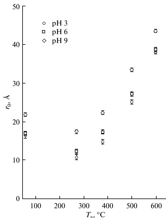
Fig. 7. Maximal size of individual particles r_0 vs. annealing temperature for hydrous ZrO_2 samples prepared at pH of (1) 3, (2) 6, and (3) 9.
