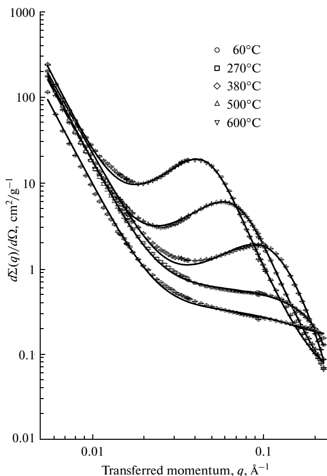
Fig. 3. Differential SANS cross section d\Sigma(q)/d\Omega for the xerogel prepared at pH 6 and its annealing products.
