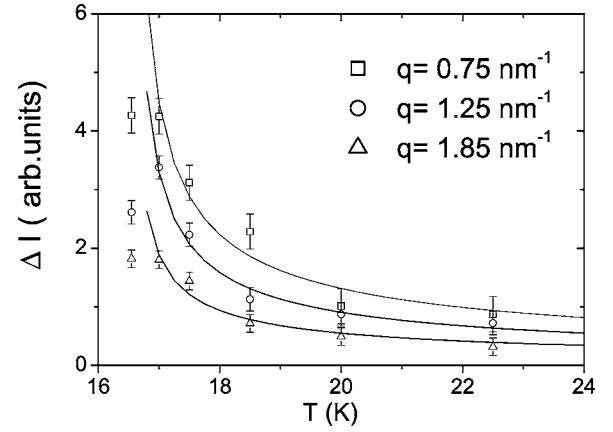
FIG. 9. Temperature dependence of \langle \Delta I \rangle for three different q values q=0.75 \text{ nm}^{-1} , q=1.25 \text{ nm}^{-1} , and q=1.85 \text{ nm}^{-1} in a field H=50 mT.
